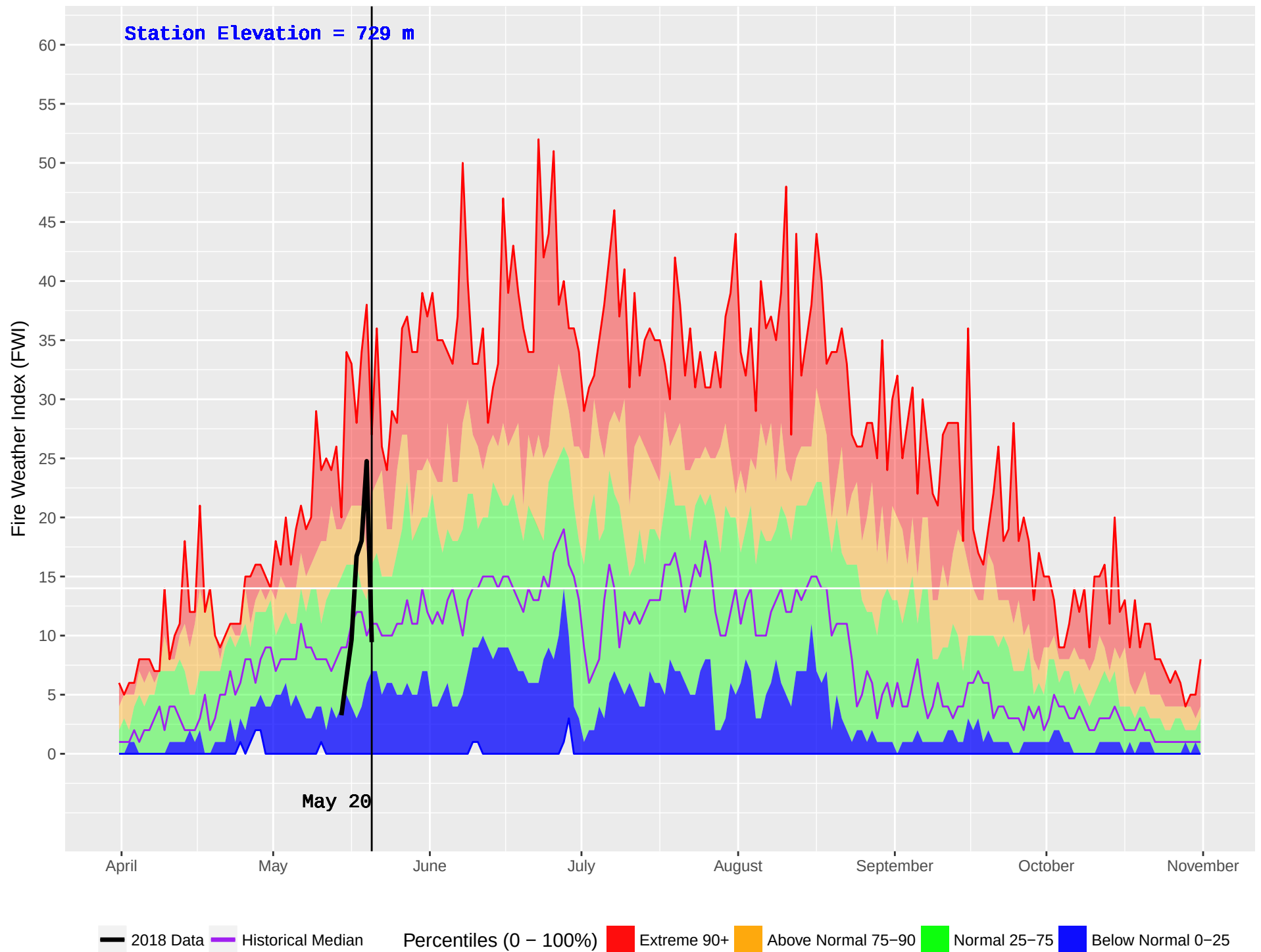
ATLIN (111) : Historical (1977–2016) and Current (2018) Noon Fire Weather Index (FWI)
